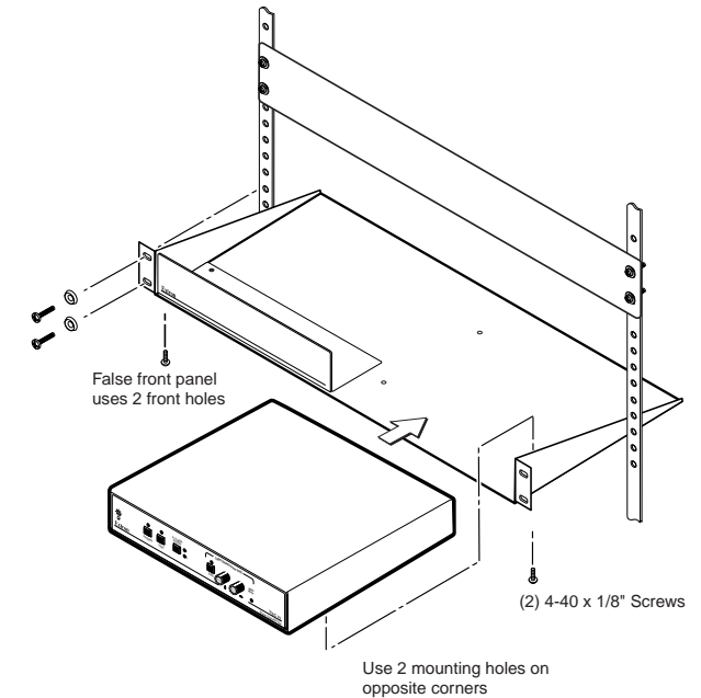
Figure 2 — Rack mounting
