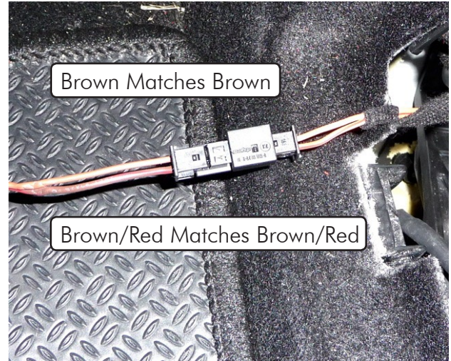
Plugs matched up and completed
