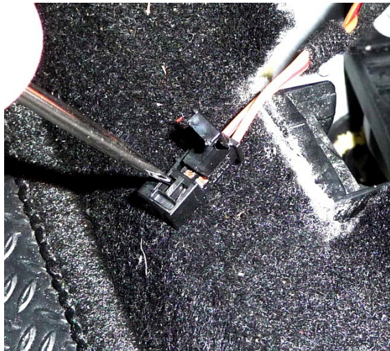
Remove pins from connector housing
