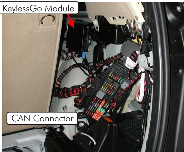
GL -- right rear side of cargo compartment
