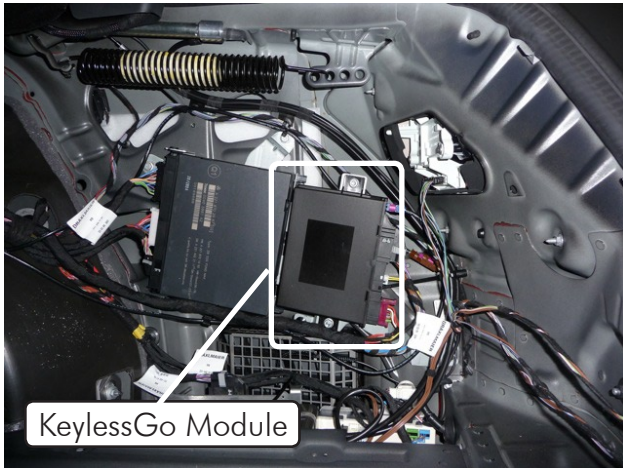
Right rear corner of trunk
