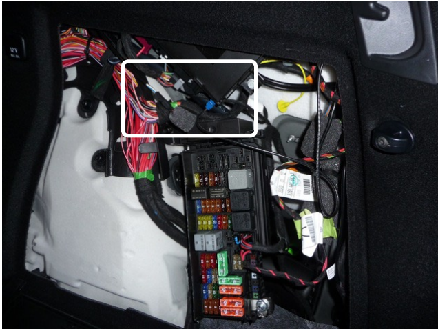
ML KeylessGo -- right rear side of cargo compartment
