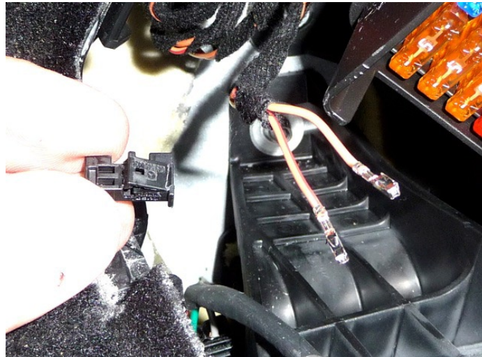
Pins removed, connector housing empty
