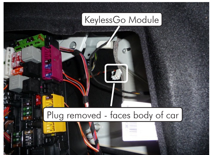
C and E Sedan KeylessGo module -- right rear trunk
