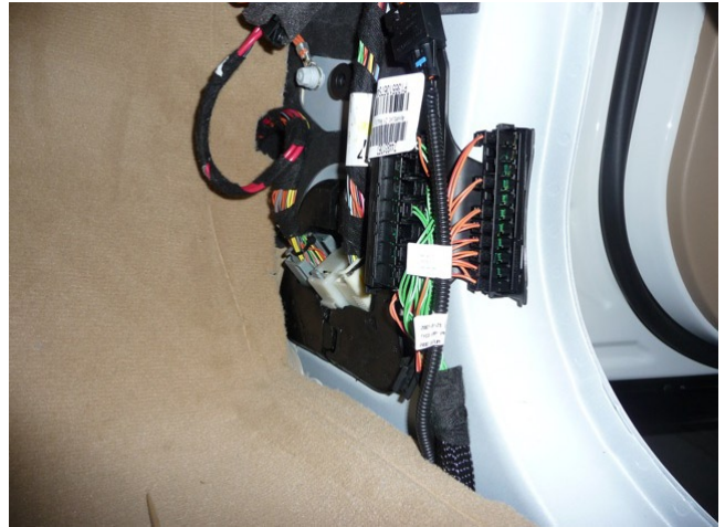
ML and R CAN distribution block, front passenger kick panel
