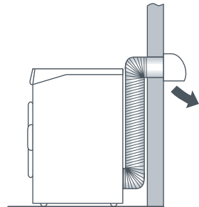
Fig. 5 External venting
