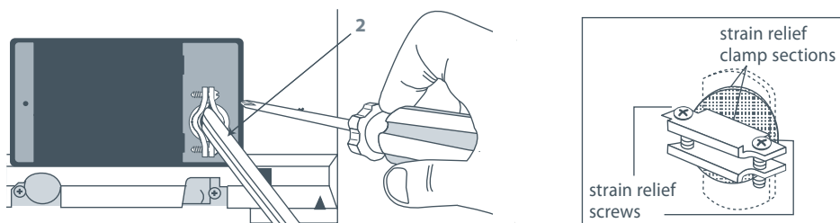
Fig.27 Inserting the power cord
