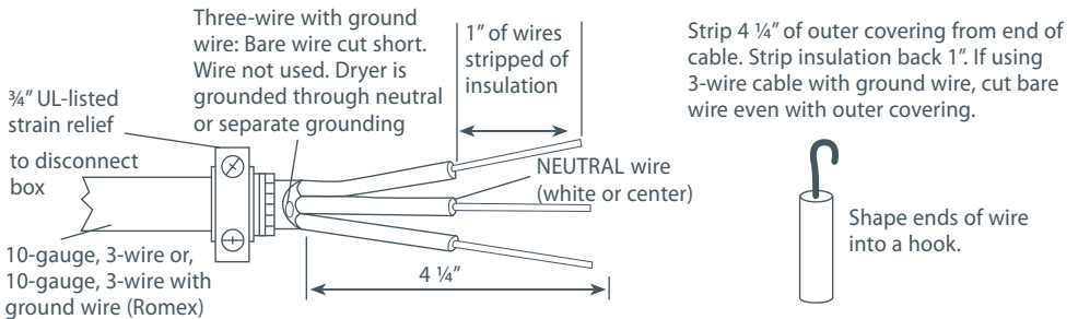
Fig.21 Wiring 3-wire connections
