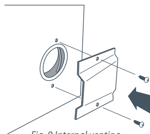
Fig. 9 Internal venting
