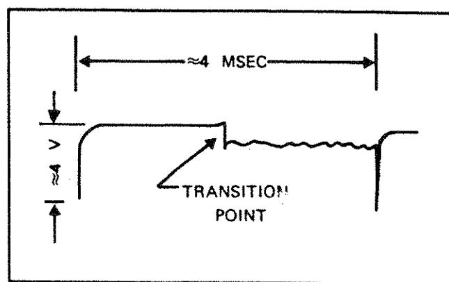
Figure 4-9. CHOPPER WAVEFORM
