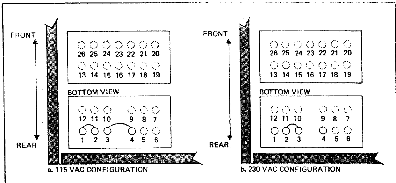
Figure 4-4 115/230 VAC CONVERSION
