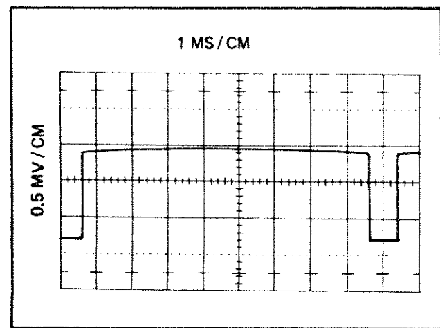
Figure 4-11. PRE - REGULATOR Q1, WAVEFORM ON OPR
