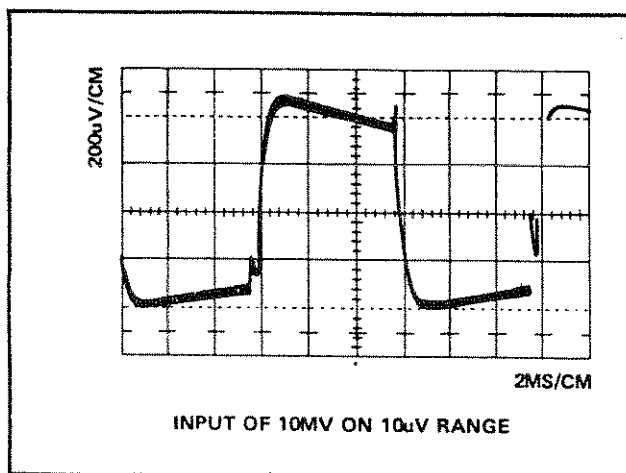
Figure 4-18. WAVEFORM AT EMITTER OF Q3
