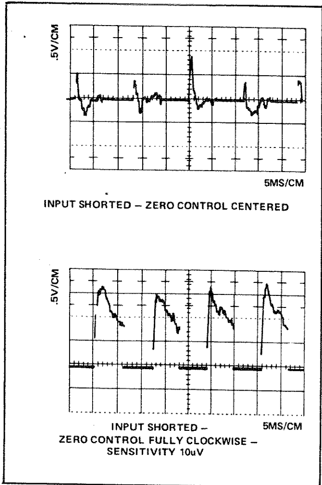
Figure 4-14. WAVEFORMS AT EMITTER OF Q6
