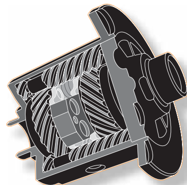
Torsen ® Limited-Slip Rear Differential – Standard on FX4 LEVEL II, this is a full-time, torque-sensing, torque-biasing system.
