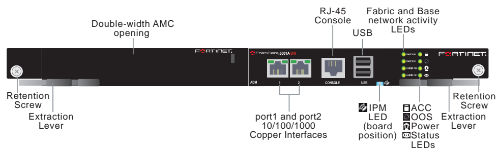
Figure 2: FortiGate-5001A-SW front panel
