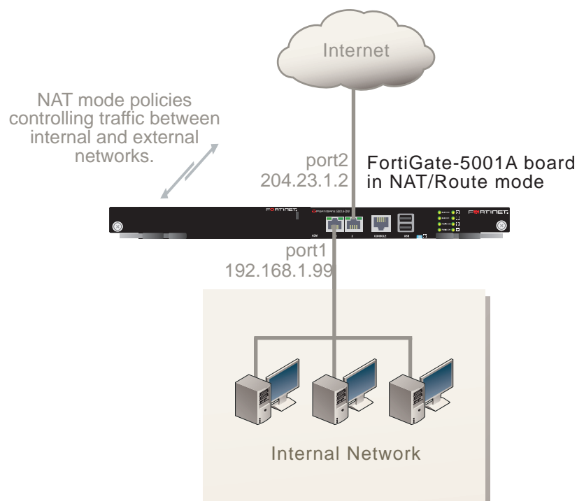
Figure 11: Example FortiGate-5001A board operating in NAT/Route mode
