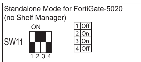
Figure 7: FortiGate-5020 setting for SW11 (standalone mode)
