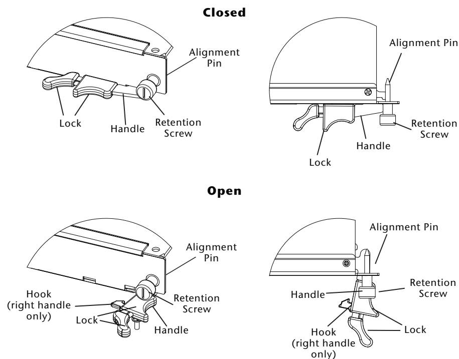
Figure 9: FortiGate-5001A right (bottom) mounting components
