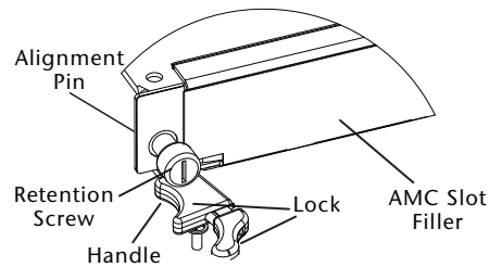
Figure 10: FortiGate-5001A-DW left (top) mounting components
