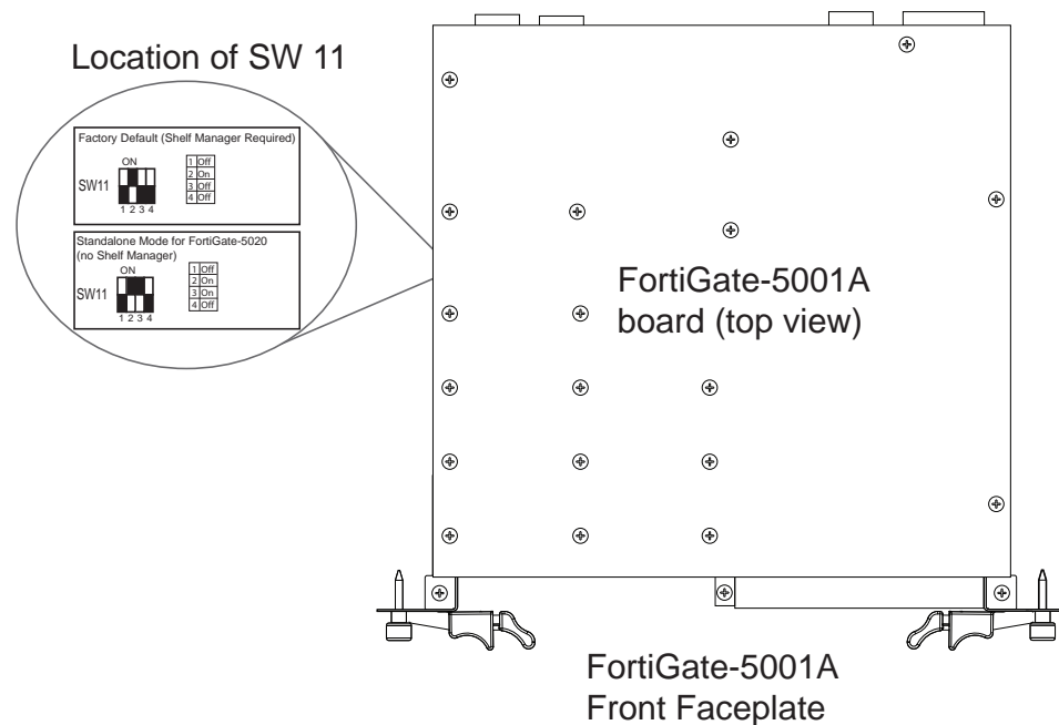
Figure 8: Location of SW11 on the FortiGate-5001A board
