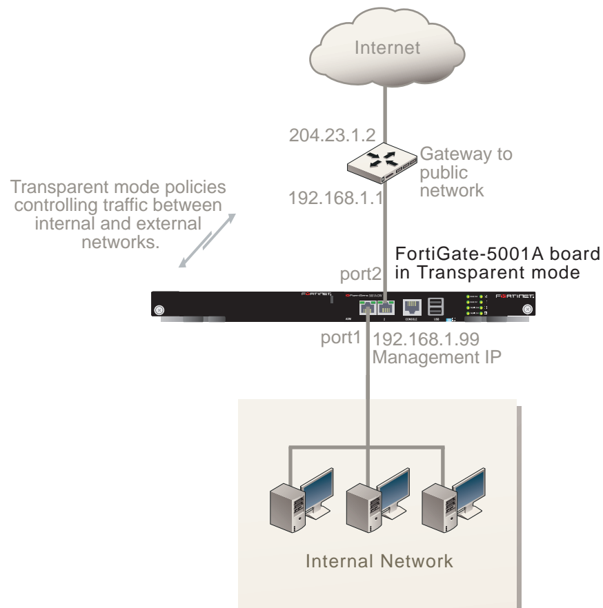
Figure 12: Example FortiGate-5001A board operating in Transparent mode
