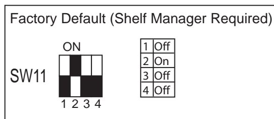
Figure 6: FortiGate-5140 and 5050 setting for SW11 (factory default shelf manager mode)
