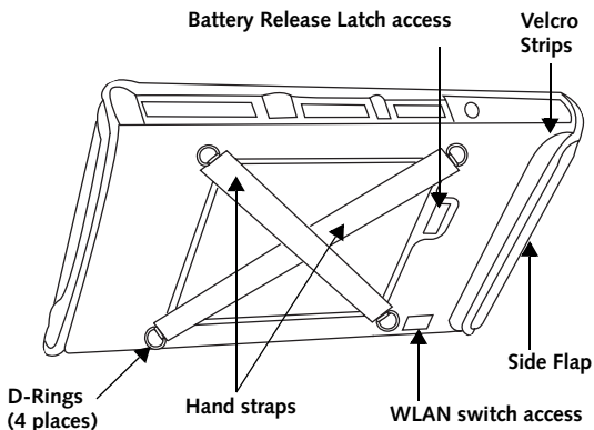
Figure 2. Bump case - Rear
