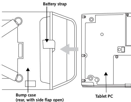
Figure 3. Inserting Tablet PC into Bump Case
