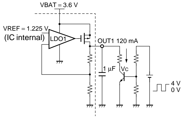
[Measurement diagram]
