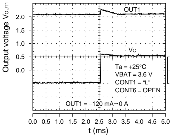
Waveform at rapid change of output load (LDO1)
