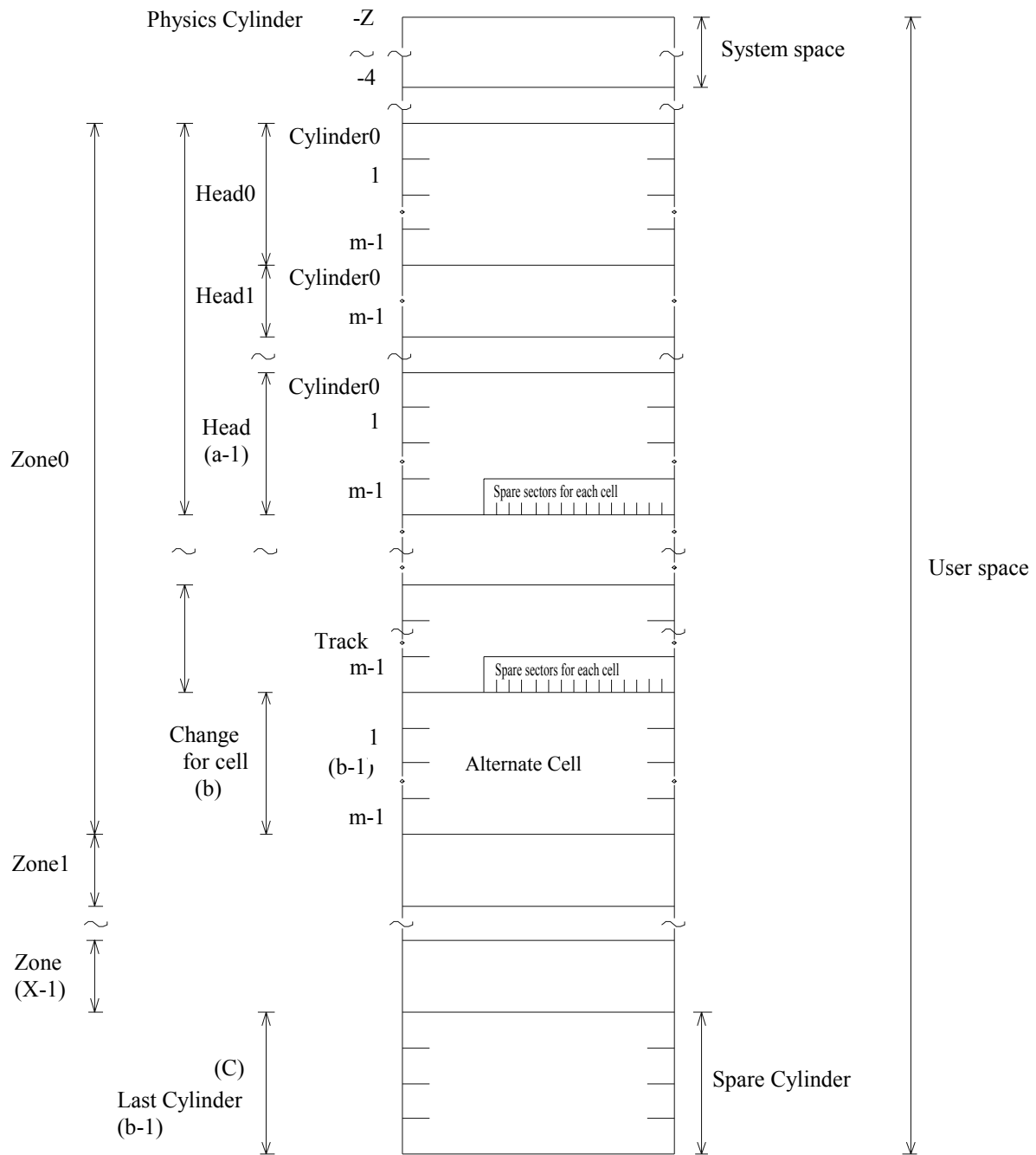
Figure 3.1 Cylinder configuration
