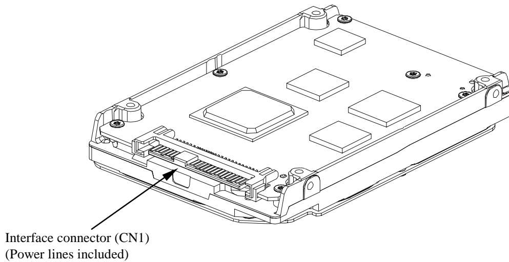
Figure 4.9 Connector location
