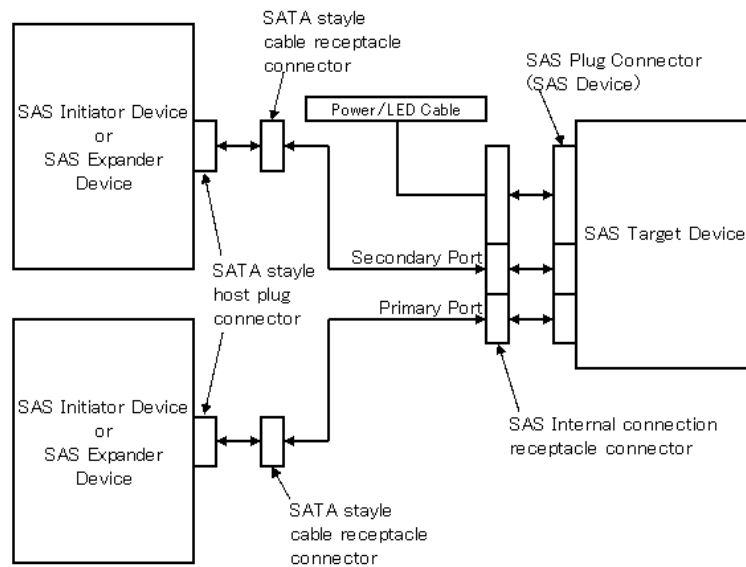
Figure 1.1 Example of SAS system configuration (Dual port internal cabled environment)
