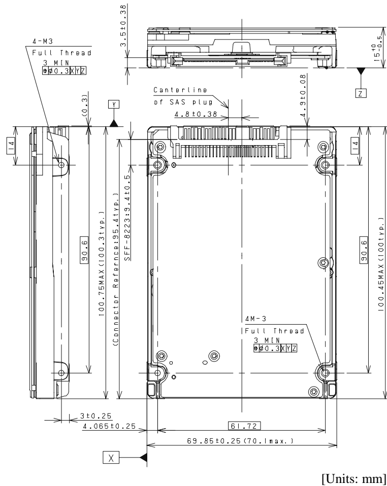
Figure 4.1 Dimensions
