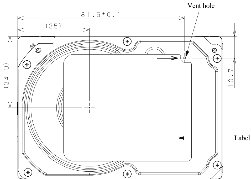
Figure 4.4 Vent hole location
