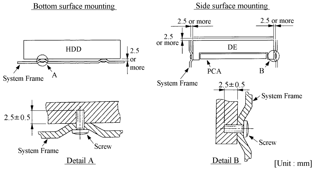
Figure 4.3 Mounting frame structure example
