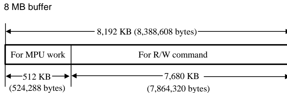
Figure 6.5 Data buffer structure
