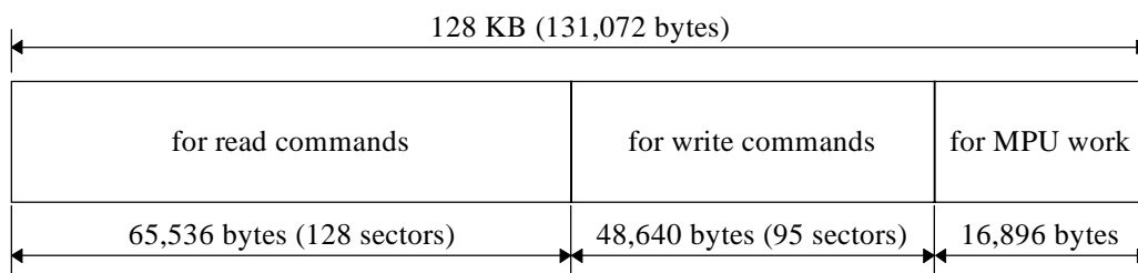
Figure 6.9 Data buffer configuration
