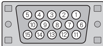
mD-sub input terminal (RGB1 INPUT/mD-sub)
