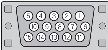
mD-sub input terminal (RGB1 INPUT/mD-sub)
