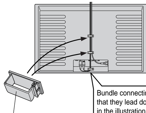
Cable clamer (Attach as in the illustration.)
