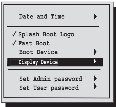
Figure 2. Startup Menu
