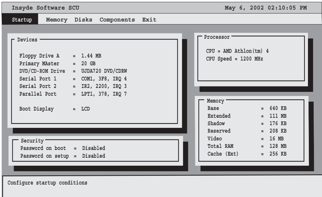
Figure 1. Main Menu
