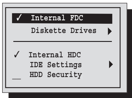
Figure 9. Disks Menu
