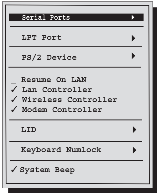
Figure 11. Components Menu
