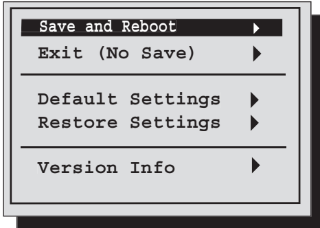
Figure 17. Exit menu
