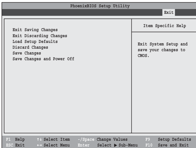
Figure 18. Exit Menu
