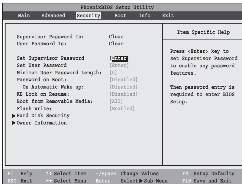
Figure 12. Security Menu
