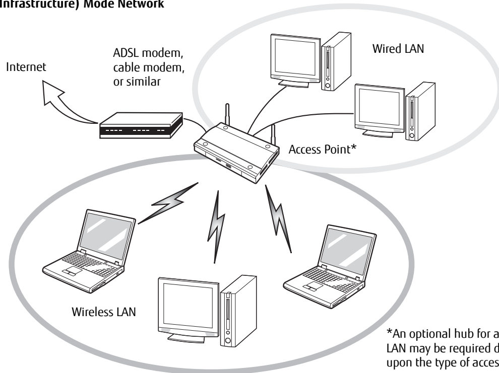
Access Point (Infrastructure) Mode Network
