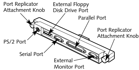
Figure 4-2 Port Replicator Rear Panel
