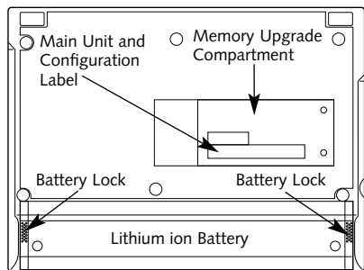
Figure 1-9 LifeBook B Series Bottom
