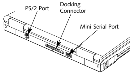
Figure 1-8 LifeBook B Series Rear Panel
