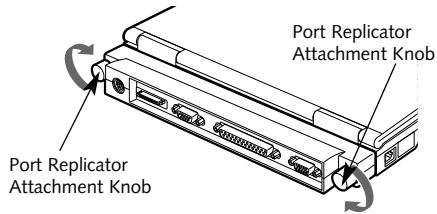
Figure 4-4 Securing the Connection
