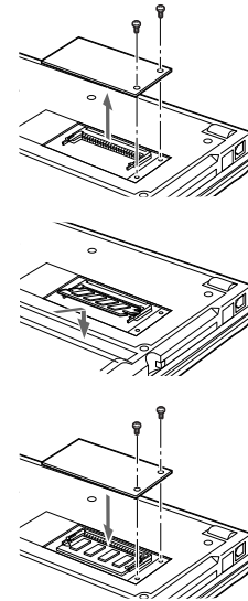
Figure 4-10 Memory Upgrade Installation
