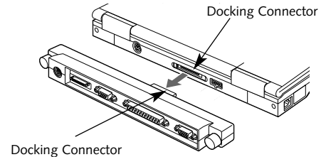
Figure 4-6 Removing the Port Replicator
