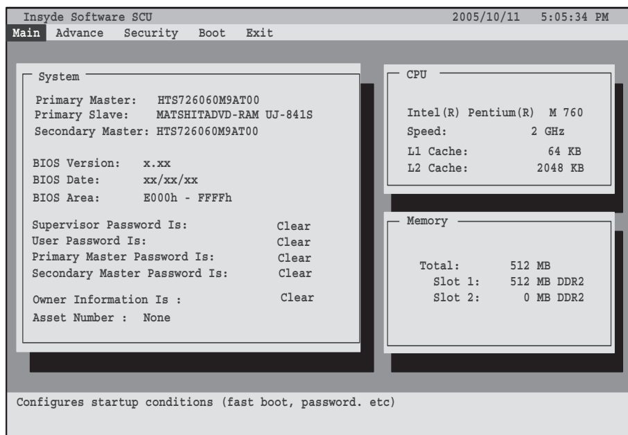
Figure 1. Information Menu
