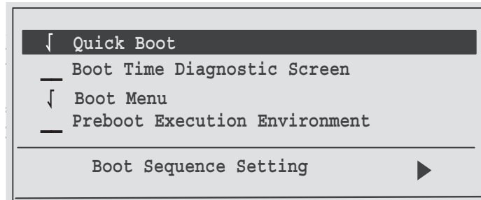
Figure 17. Boot Menu
