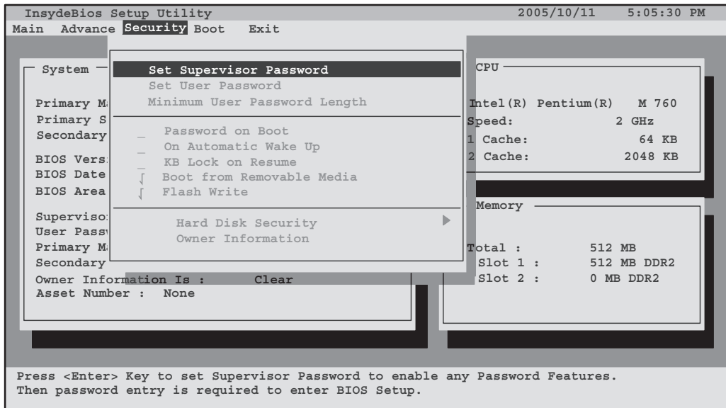
Figure 13. Security Menu
