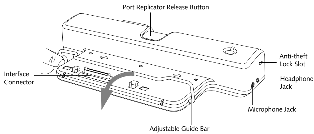
Figure 4-12. Port Replicator front panel
