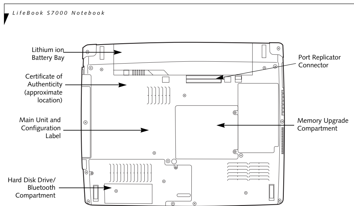
Figure 2-7. LifeBook notebook bottom panel
