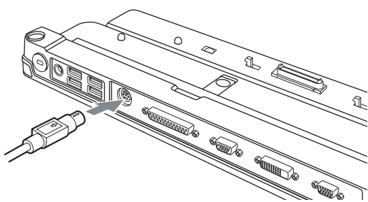
Figure 4-24. Connecting a PS/2 Device
