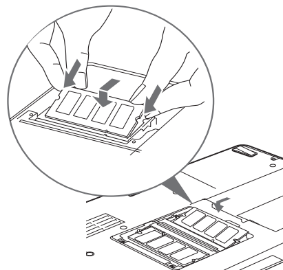
Figure 4-11. Installing a Second Memory Module
