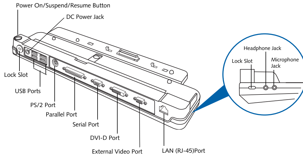
Figure 4-16. Port Replicator back side
