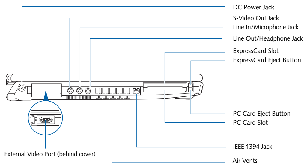
Figure 2-5. LifeBook notebook left-side panel
