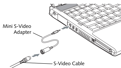
Figure 4-26. Connecting the S-Video Cable Adapter
