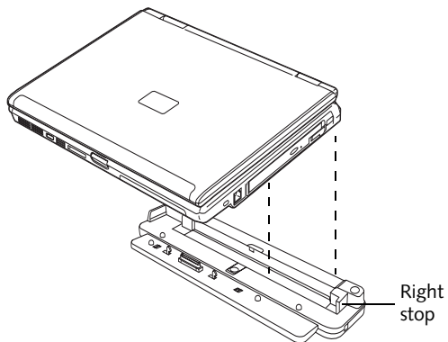
Figure 4-19. Aligning the notebook
