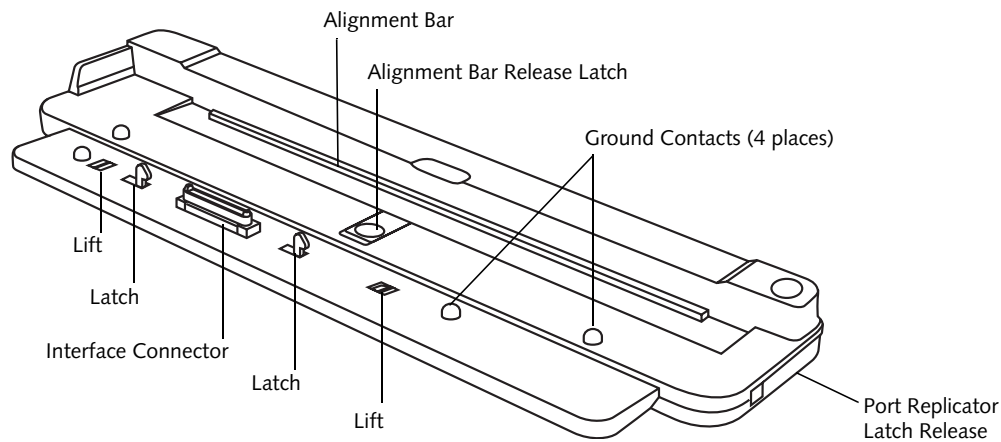
Figure 4-17. Port Replicator front side
