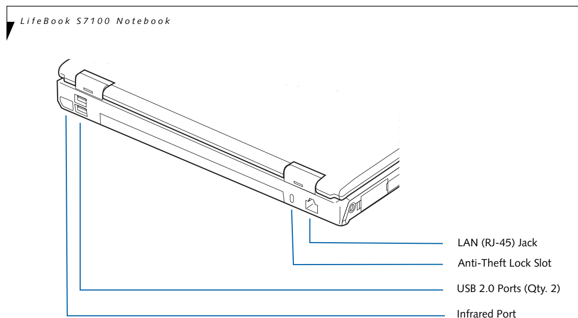
Figure 2-7. LifeBook notebook back panel
