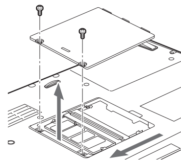
Figure 4-10. Opening the Memory Upgrade Compartment
