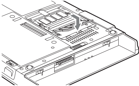
Figure 2-9. Installing a DIMM Module
