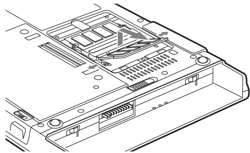
Figure 2-10. Removing a DIMM Module
