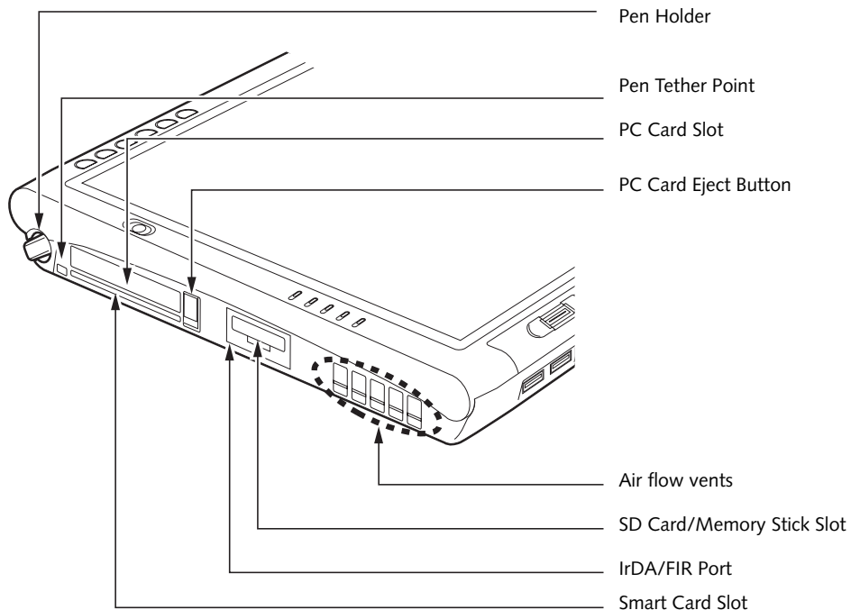
Figure 1-4. Stylistic ST5100 Series Tablet PC Features (Top View)
