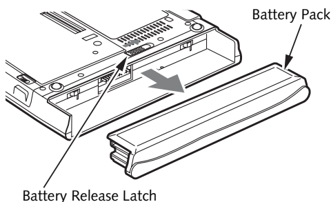
Figure 2-4. Removing the Battery
