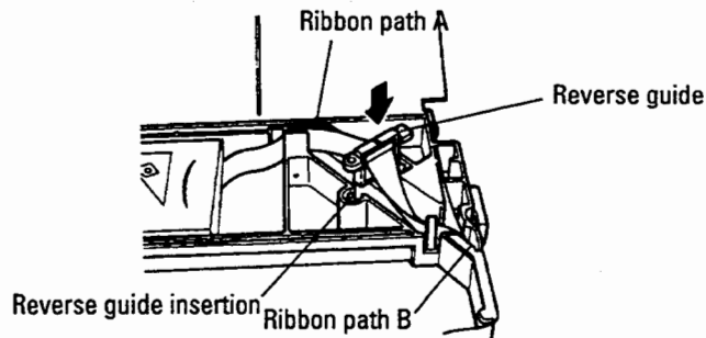
Figure 3-9 Ribbon paths (1)
