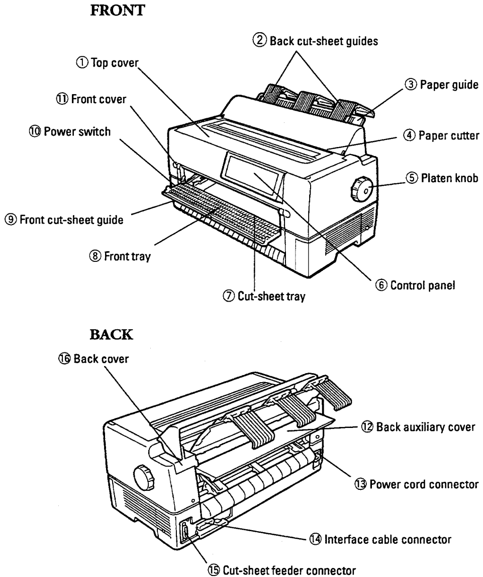
Figure 1-3 Parts (1)
