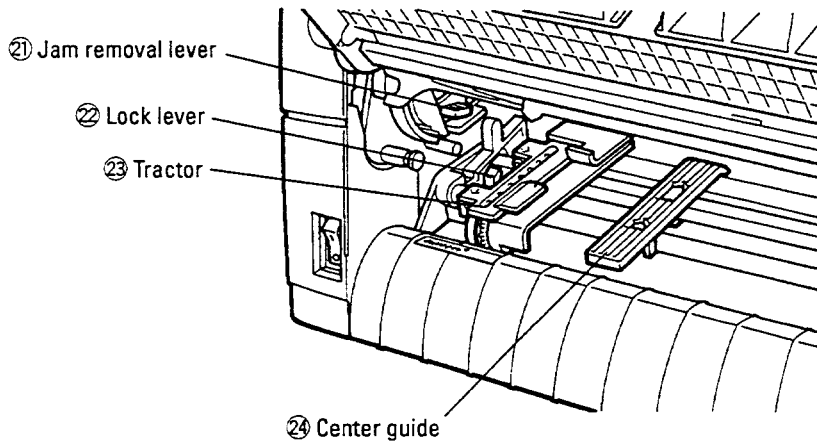
Figure 1-4 Parts (2)
