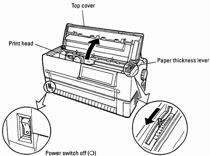
Figure 3-2 Installing the ribbon cassette (1)
