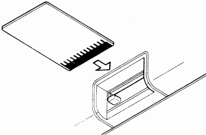
Figure 3.14 IC Card and Card Slot
