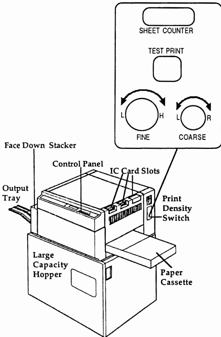
Figure 1.1 Laser Printer
