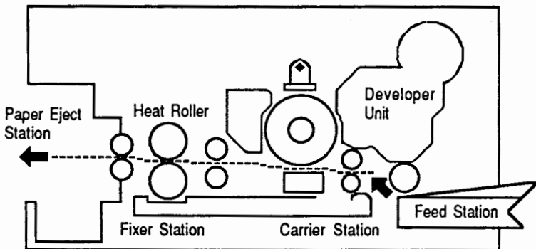
Figure 8.1 Paper Route
