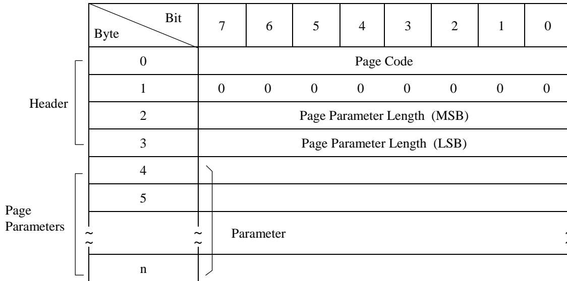
Figure 3.21 RECEIVE DIAGNOSTIC RESULTS command: Response data configuration
