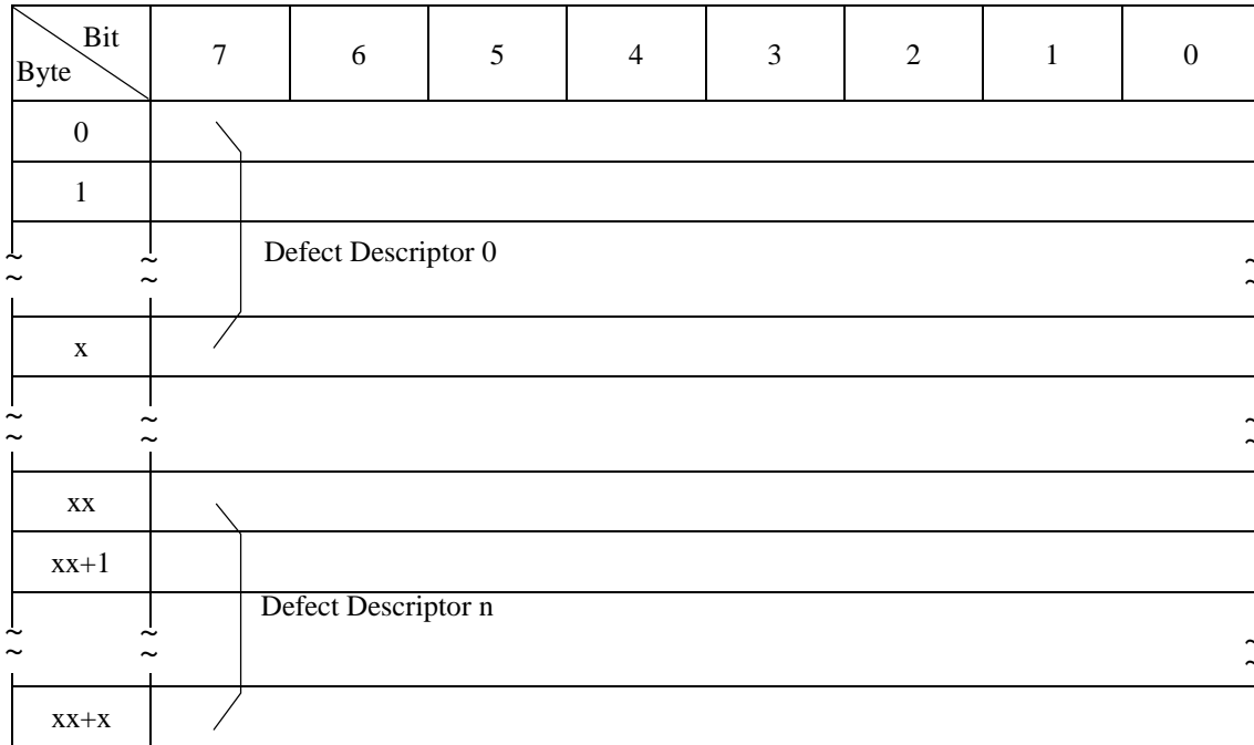
Figure 3.13 FORMAT UNIT command parameter list configuration
