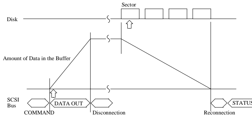
Figure 2.3 Example of data buffer operation during write
