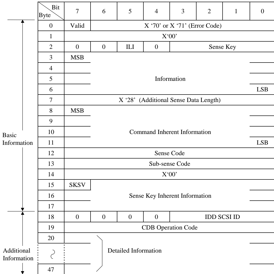
Figure 5.1 Expanded sense data format
