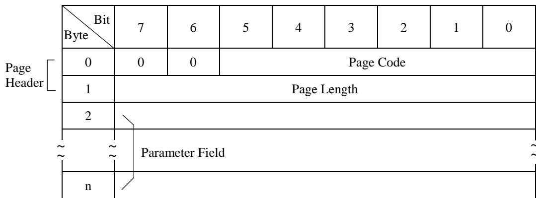
Figure 3.10 MODE SENSE command (Group 0) parameter configuration
