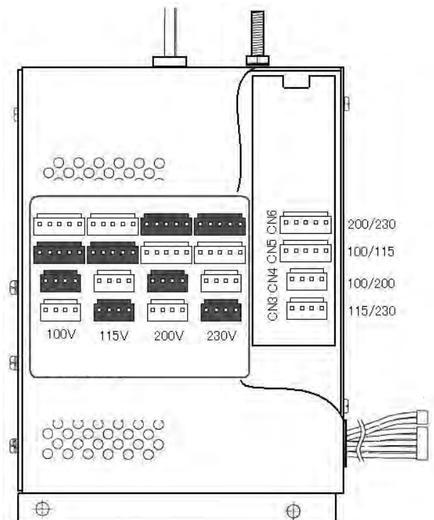
Fig. 4.2.3 AC power supply unit
