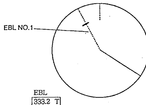
Figure 11b How to Measure True Bearing with an EBL
