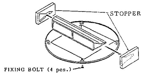
Fig.4 Removing the Radome Cover
