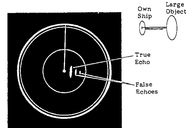
Fig.40 Multiple Echoes
