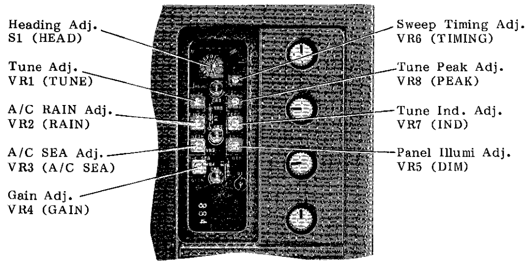
Potentiometer Compartment
