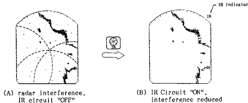
Fig.29 Radar Interference
