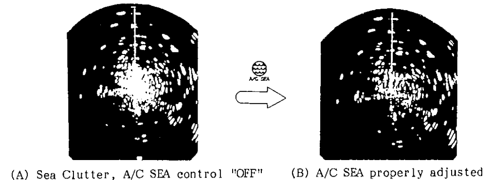
Fig.24 Adjusting the A/C SEA
