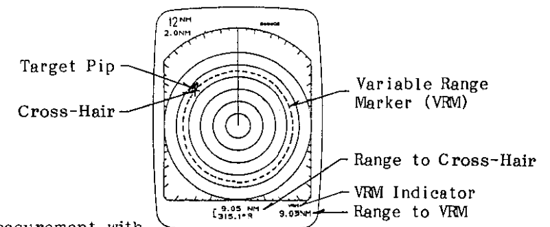
Fig.26 Range Measurement with Cross-Hair and VRM
