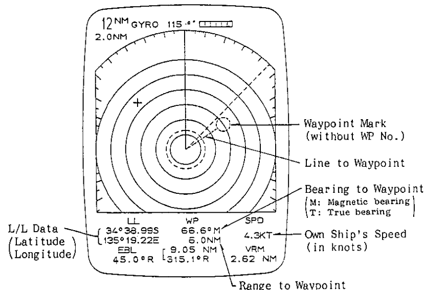
Fig.34 Nav Data on the Screen
