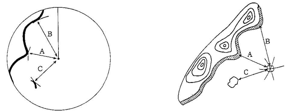
Fig.45 Position Fixing Using Radar Ranges
