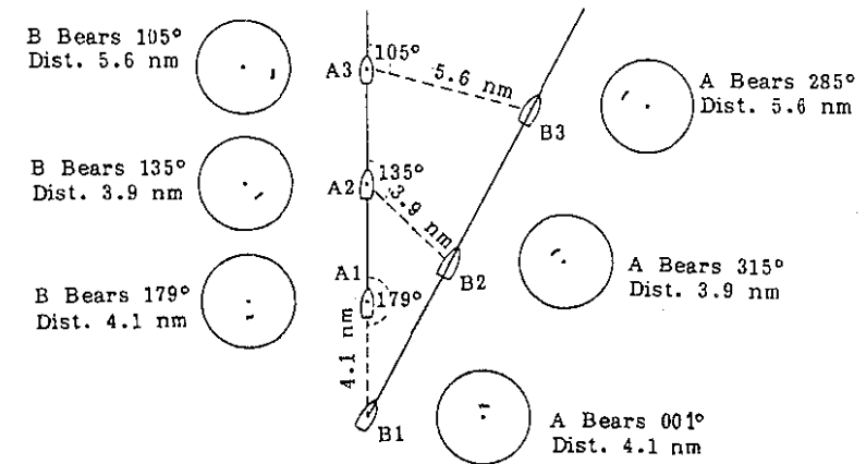
Fig.48 Relative Motion vs. True Motion
