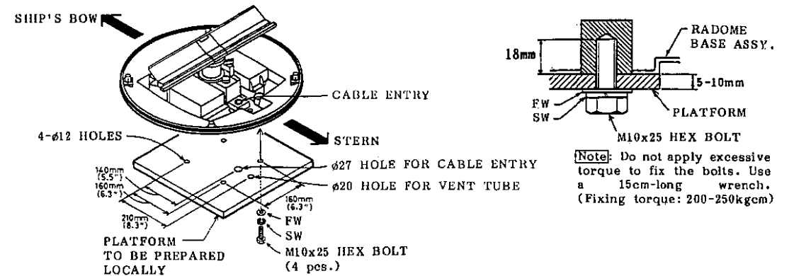
Fig.5 Installing the Scanner Unit
