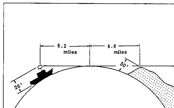
Fig.38 Radar Horizon
