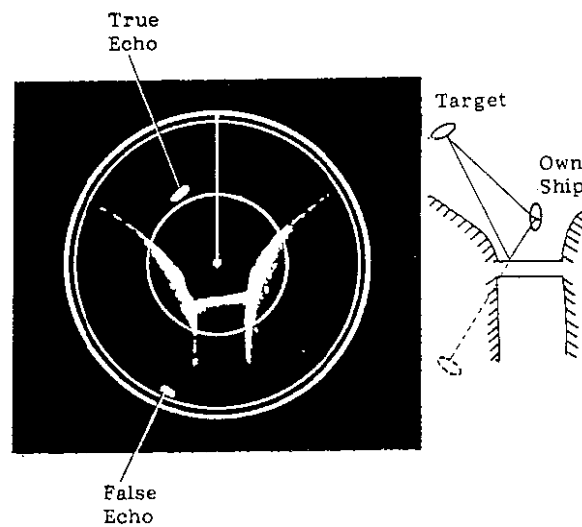
Fig.43 Indirect Echoes
