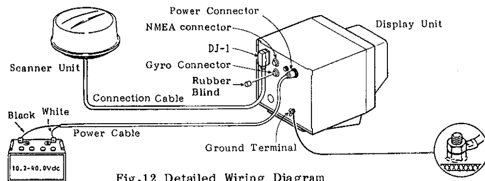
Fig.12 Detailed Wiring Diagram
