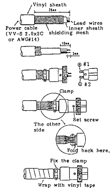
Fig.11 Power Connector Assy.
