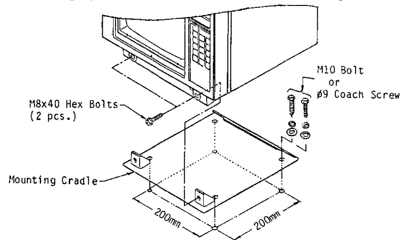
Fig.9 Tabletop Mounting
