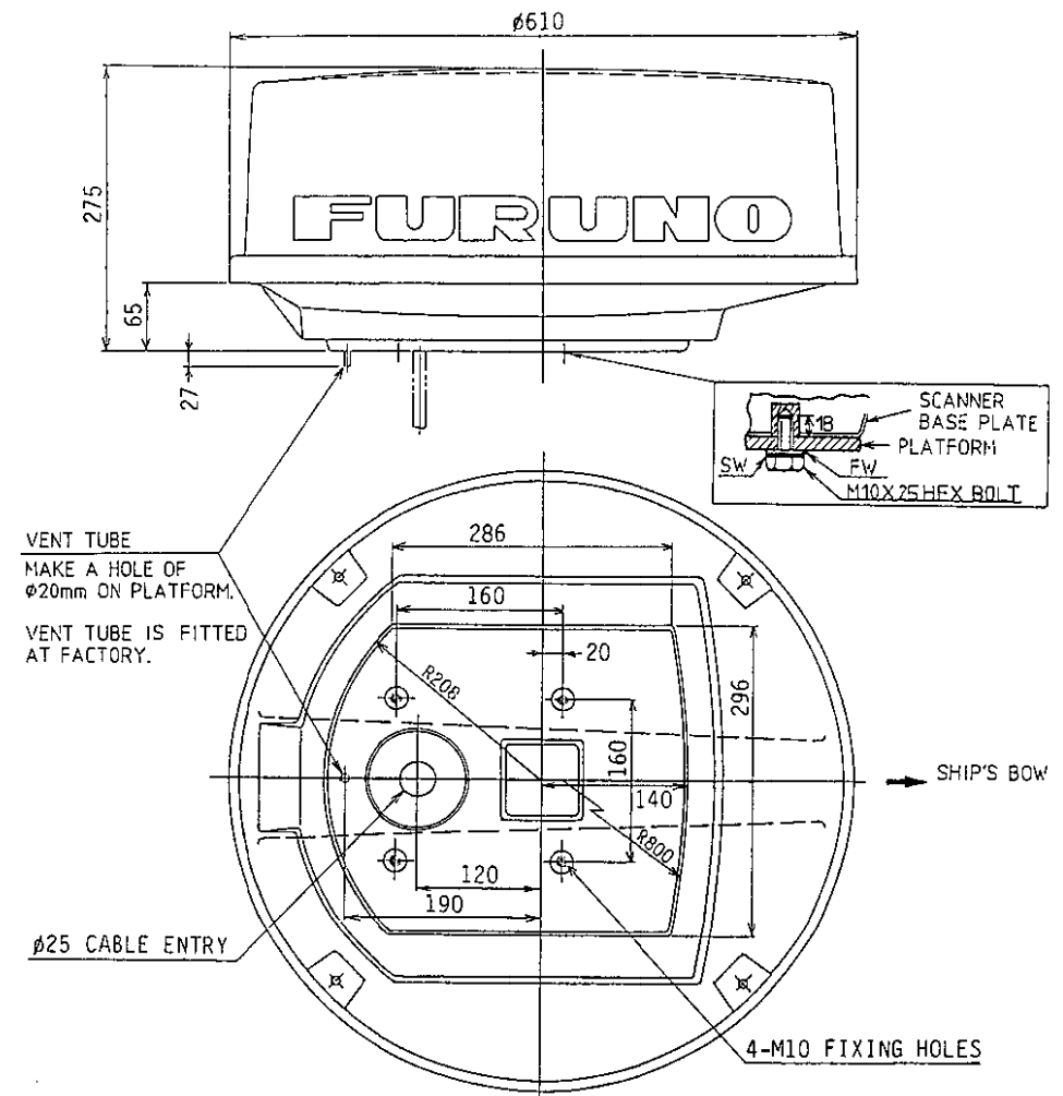
Fig.6 Scanner Unit Outline Drawing
