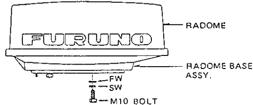
Fig.3 Preparing the Radome Base for Mounting
