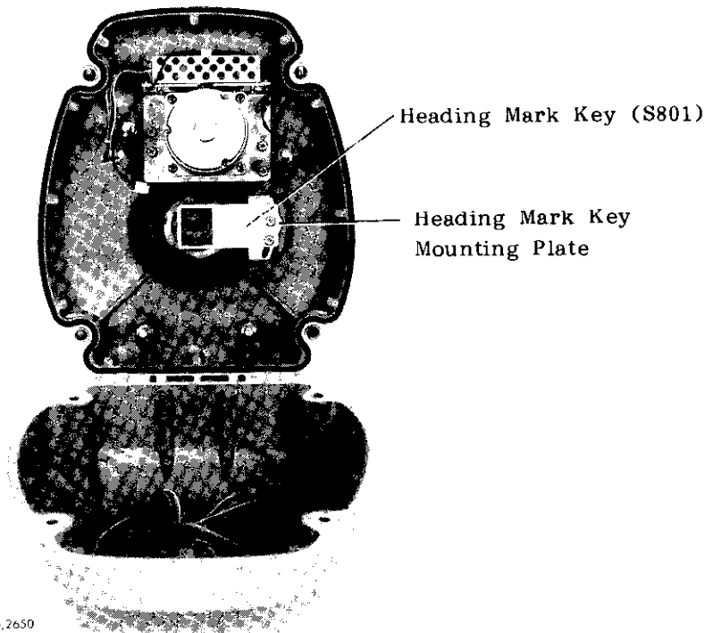
(b) Transceiver module removed
