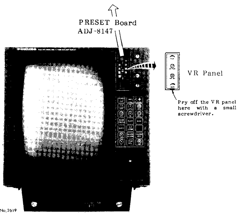
Potentiometer Compartment
