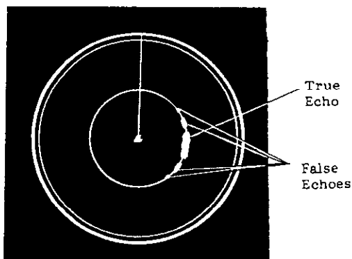
Fig.41 Side-Lobe Echoes
