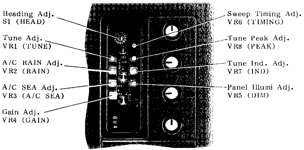
Potentiometer Compartment
