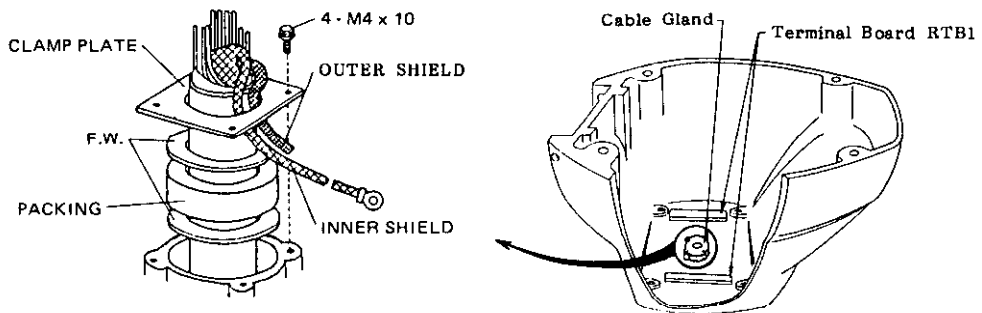
Fig.4 Bottom of Scanner Housing
