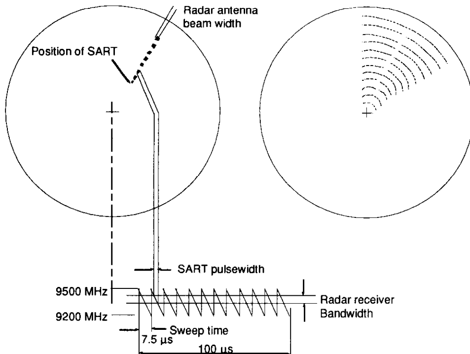
Screen A: When a distant SART is picked up
