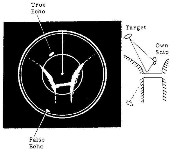
Fig.43 Indirect Echoes
