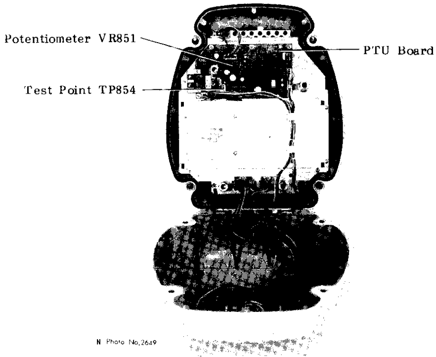
(a) Inside of scanner unit
