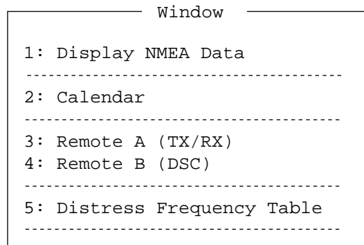
Figure 6-1 Window menu
