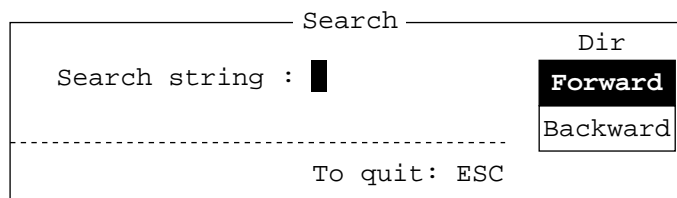
Figure 4-6 Search screen
