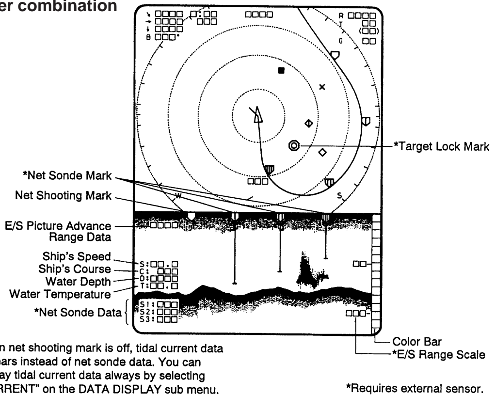
Figure 4-3 Marks and data appearing in the echo sounder display mode
