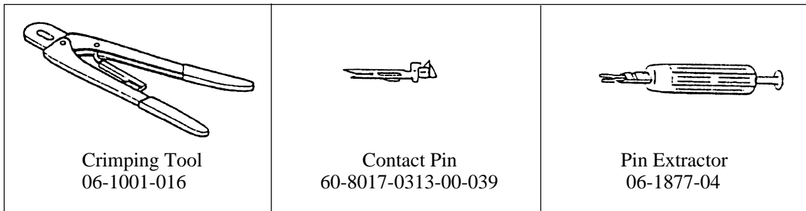
Figure 4-2a Crimping tool, contact pin, pin extractor
