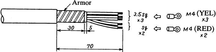
Figure 4-22 Fabricating cable 10S1259
