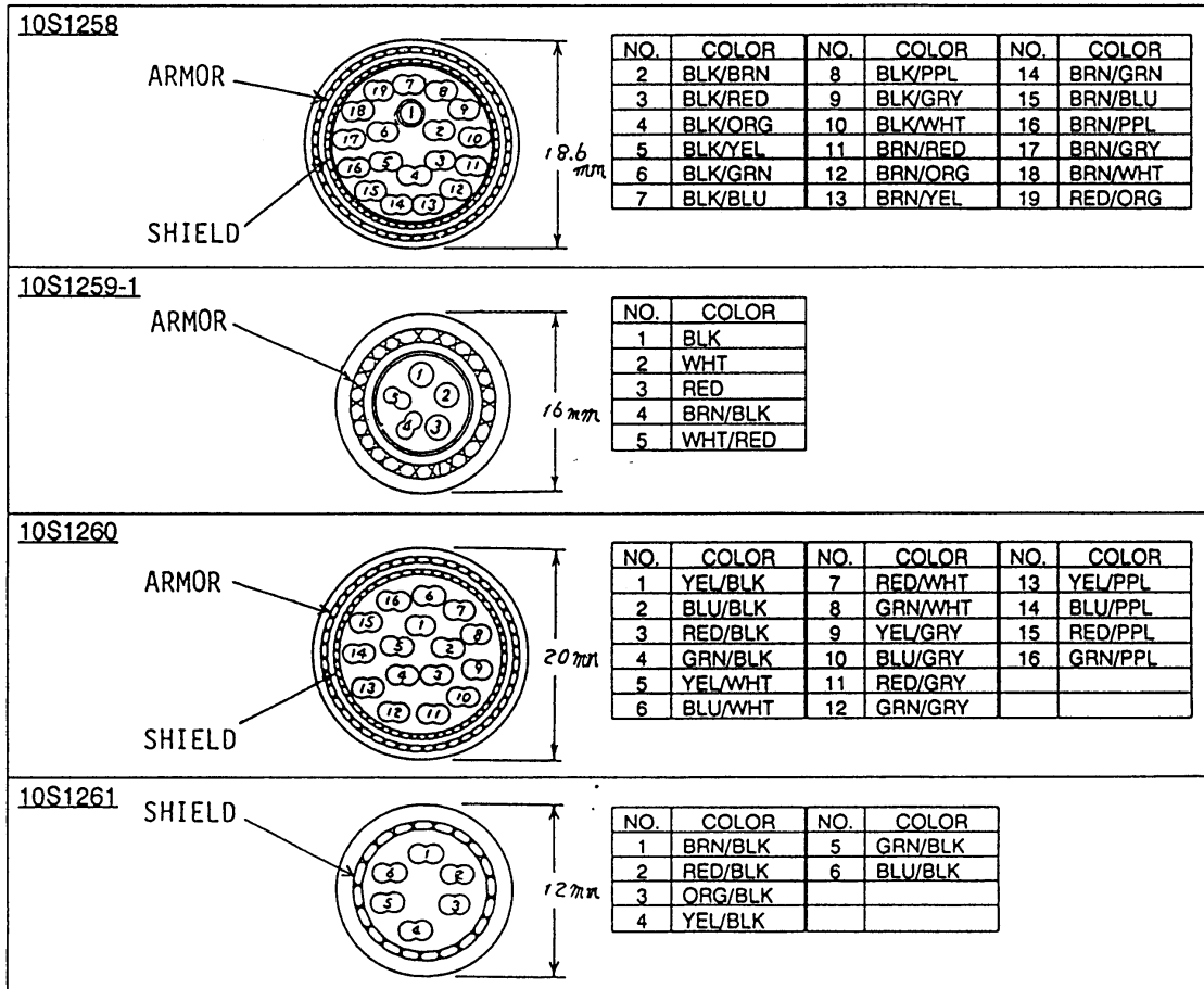
Figure 4-1 Cable configuration
