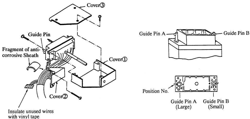
Figure 4-15 Assembling 38P connector
