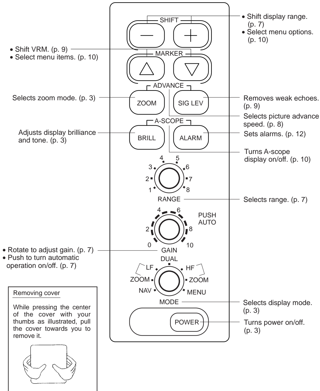
Figure 1-1 Controls
