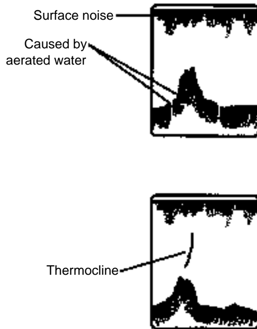
Figure 3-4 Surface noise/aeration
