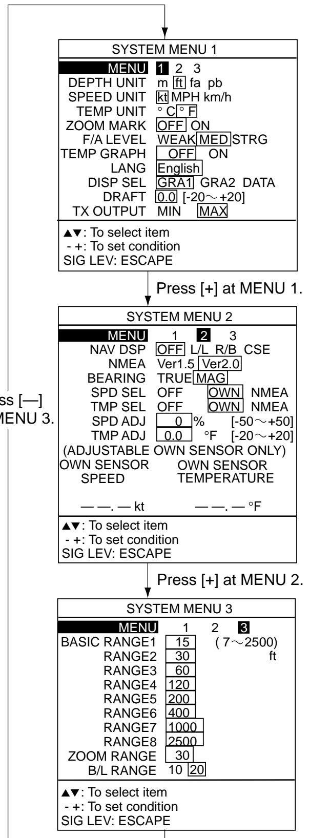
Figure 2-2 System menus
