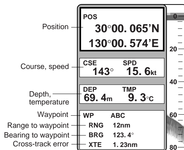
Figure 1-12 Data display
