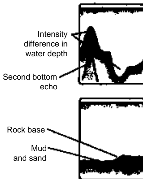
Figure 3-3 Bottom echoes
