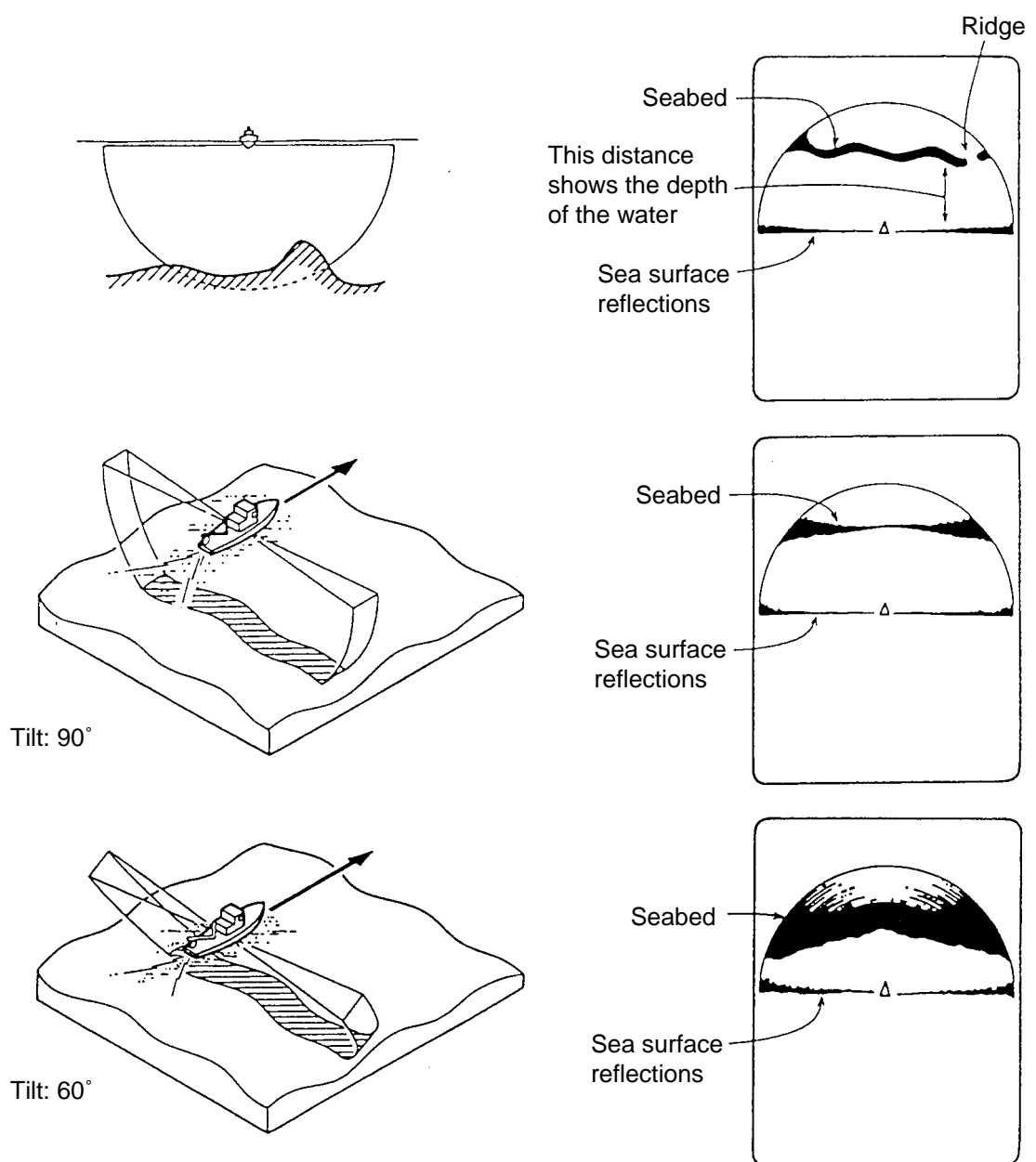
Figure 9-1 Seabed echoes
