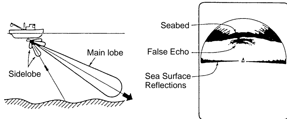
Figure 9-5 Sidelobe echoes
