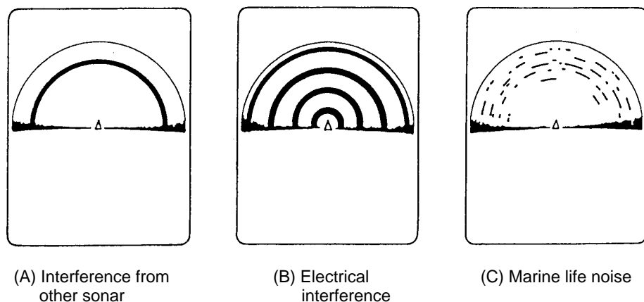
Figure 9-6 Noise and interference
