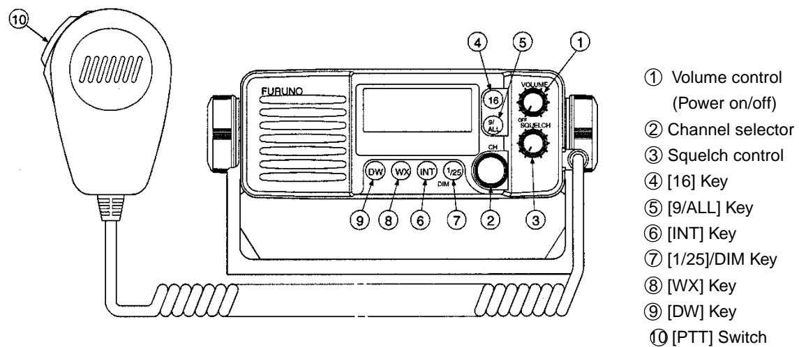
Fig. 3-1 Controls
