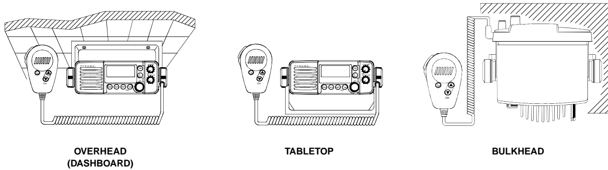
Fig. 2-1 Mounting Methods
