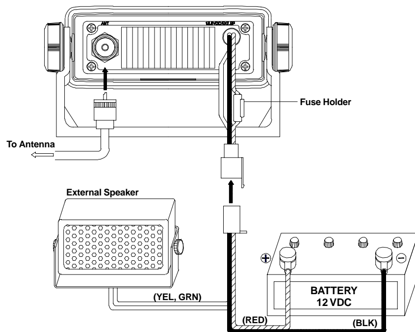
Fig. 2-3 Electrical Connections
