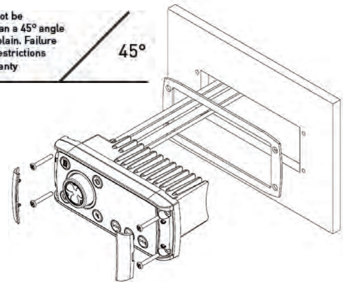
Figure 5 – Locating the RA50 unit into the mounting panel
