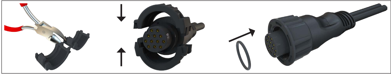
Installing a Locking Ring
