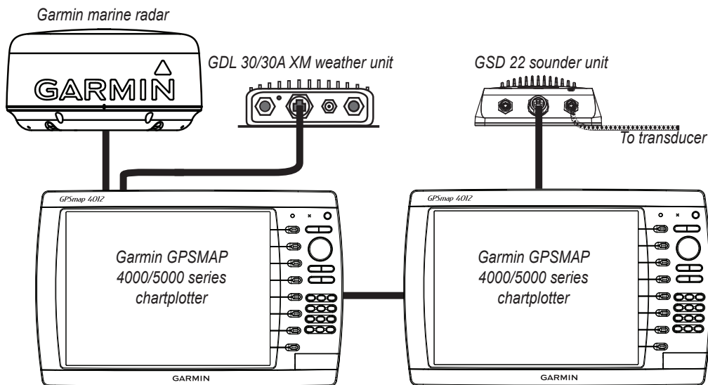
Extended Marine Network With Two Chartplotters
