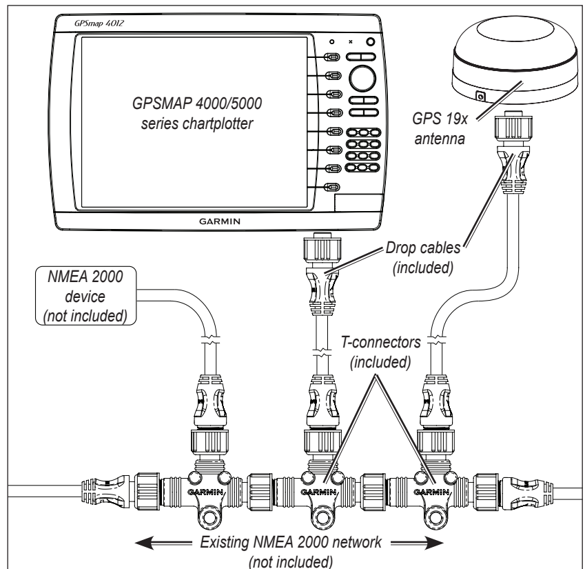
Connecting the GPSMAP 4000/5000 Series Chartplotter and GPS 19x Antenna to an Existing NMEA 2000 Network
