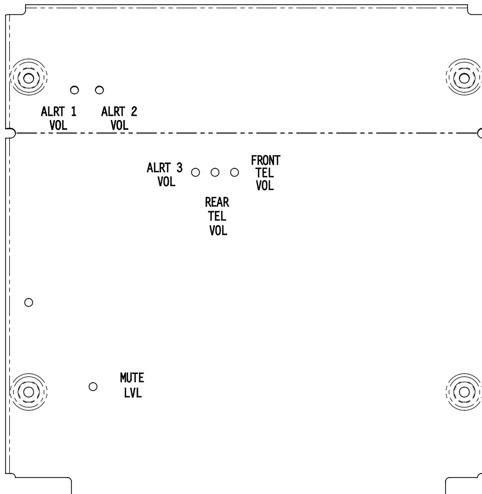
Figure 2-1. Access Hole Location (Top View)
