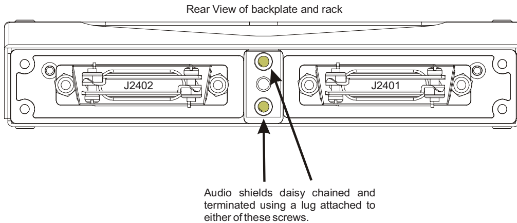
Figure 3-1. Audio Shield Termination
