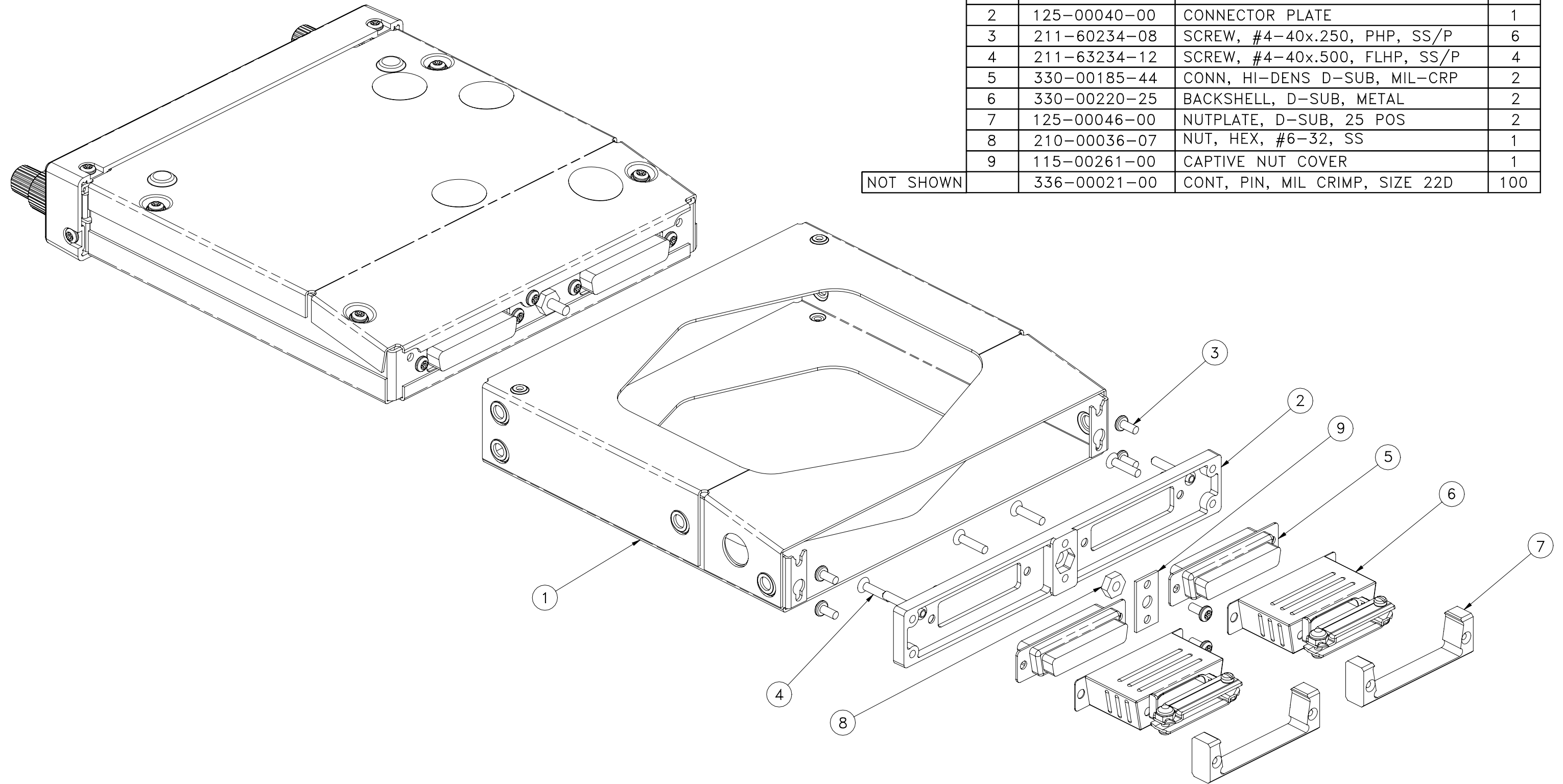
Figure A-2. GMA 240 Connector/Rack Assembly Drawing
