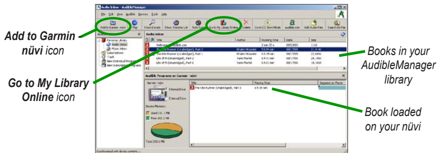
AudibleManager Program
