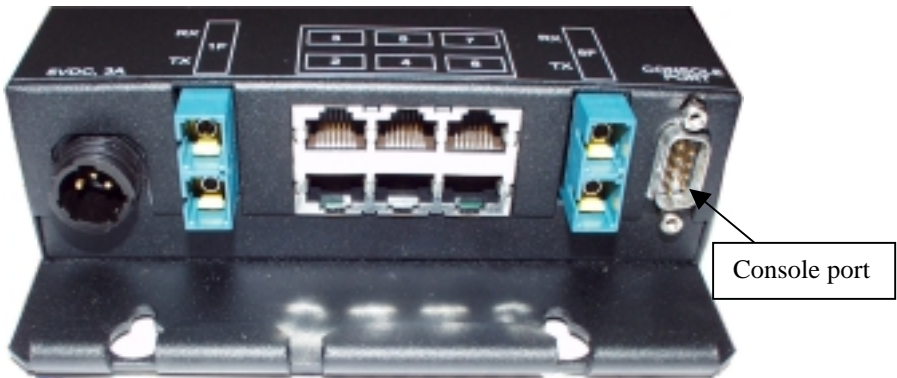
Fig. 2.2.2 Front View of Magnum mP62, Console port is located on the extreme right of the Hardened Switch
