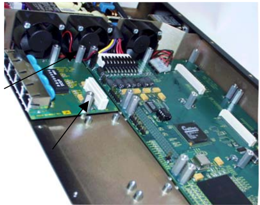
Fig 3.5.2b Granddaughter Board placed in slot A and secured with three 7/16 stand-off's
