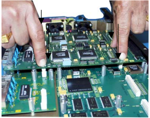
Figure 3.5.2f: Securely latching up 6KPM Cards into a Magnum 6K25e
