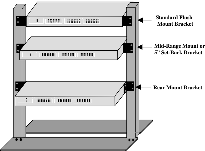
Fig 3.3.2 Reverse Magnum 6K25e units, rack-mounted in a frame
