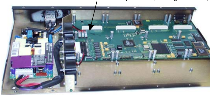
Figure 3.5.1b: Magnum 6K25e, Top view without chassis cover
