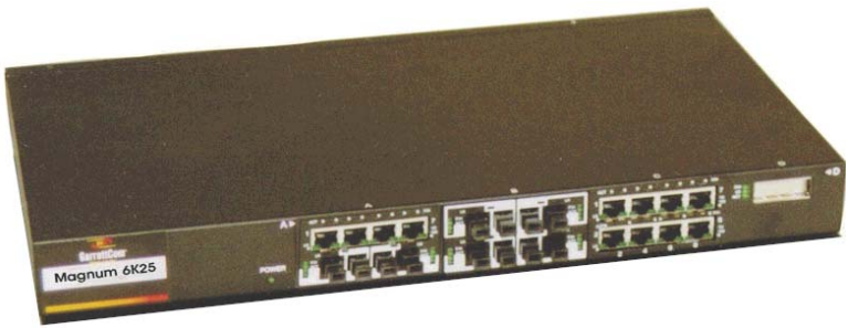
Figure 2.2.1a: “Regular” 6K25e front view, configured for 24 +1 Gb ports
