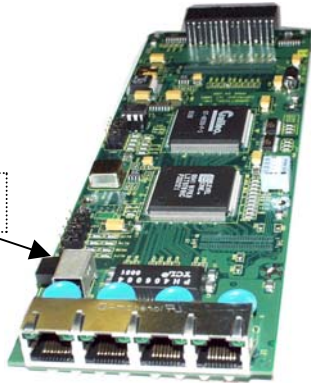
Fig. 3.5.2c Daughter Board, top view of version for 4 copper 10/100 ports. Port# 1 Can be configured as uplink (x) crossed ports for cascading as shown in the Fig.
