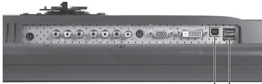
USB in ("B" type) port
