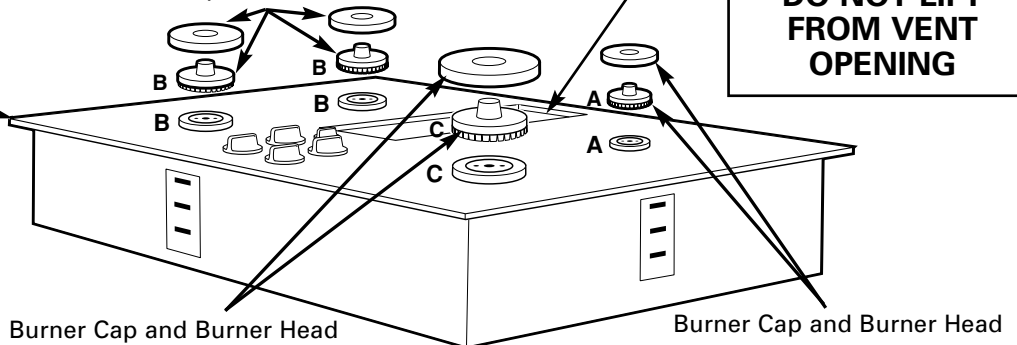
Burner Caps and Burner Heads
