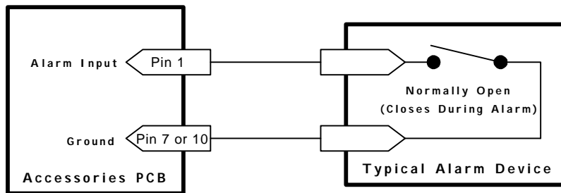
Figure 1-4 Normally Open Relay Alarm Connection
