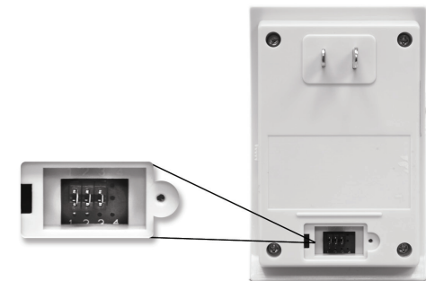
House Security Code door and jumper location
