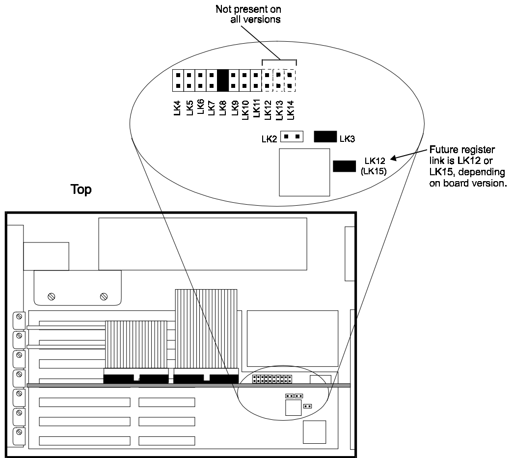
Figure 5. Jumper Locations
