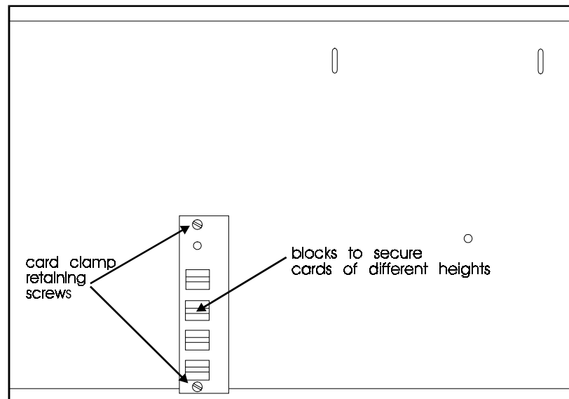
Figure 4. Card Clamp
