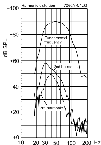
Figure 11. The curves above show the harmonic distortion analysis of the 7060A in free field. In half space the SPL will be 6 dB higher.
