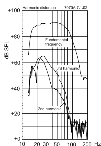
Figure 12. The curves above show the harmonic distortion analysis of the 7070A and 7071A in free field. In half space the SPL will be 6 dB higher.
