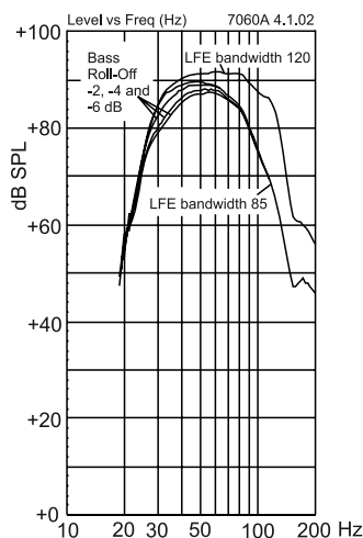
Figure 9. The free field frequency response of the 7060A subwoofer at different Bass Roll-Off settings
