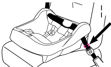
Locking clip goes here, \frac{1}{2} inch from the buckle
